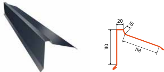
Firstblech Pultdach
